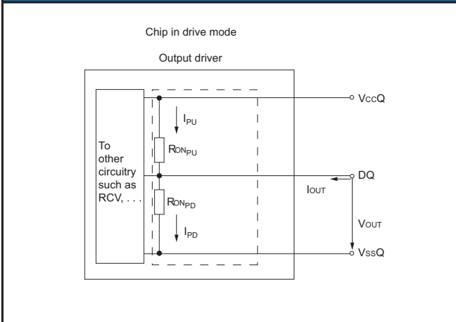
FIGURE 19 - OUTPUT DRIVER
