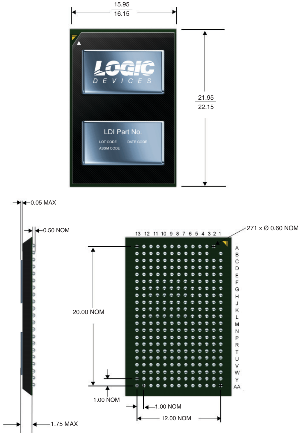
FIGURE 5 - MECHANICAL DRAWING
