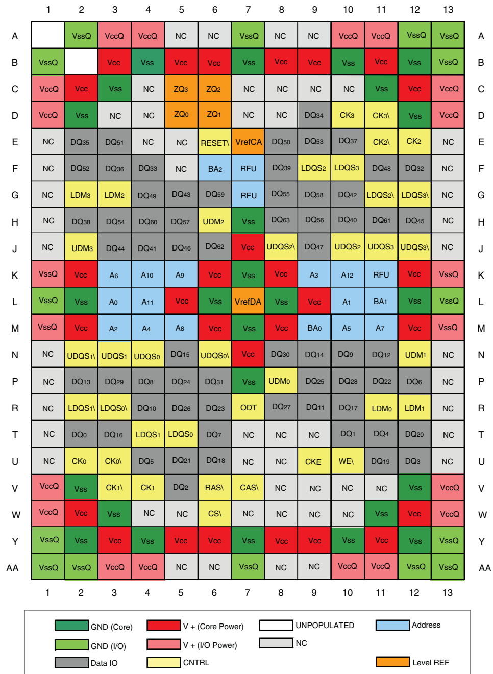
FIGURE 4 - SDRAM - DDR3 PINOUT TOP VIEW
