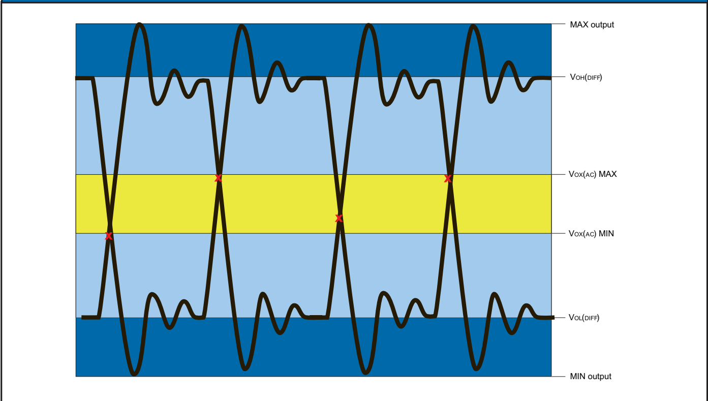
FIGURE 21 - DIFFERENTIAL OUTPUT SIGNAL
